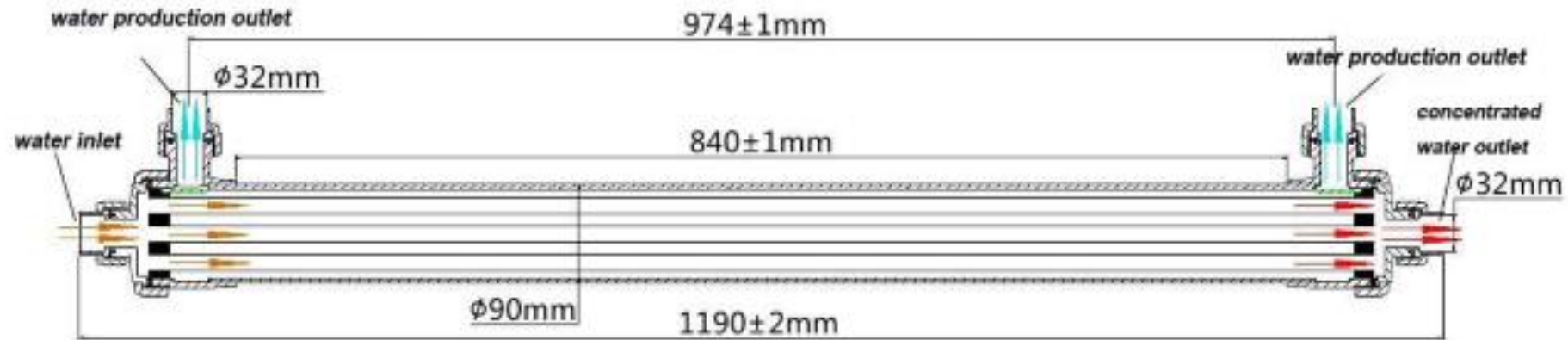
Water production flow schematic diagram
